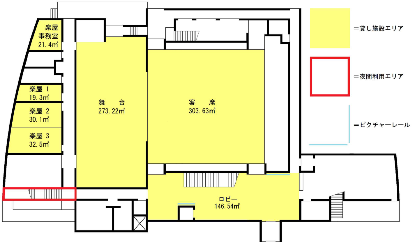
1ST FLOOR
